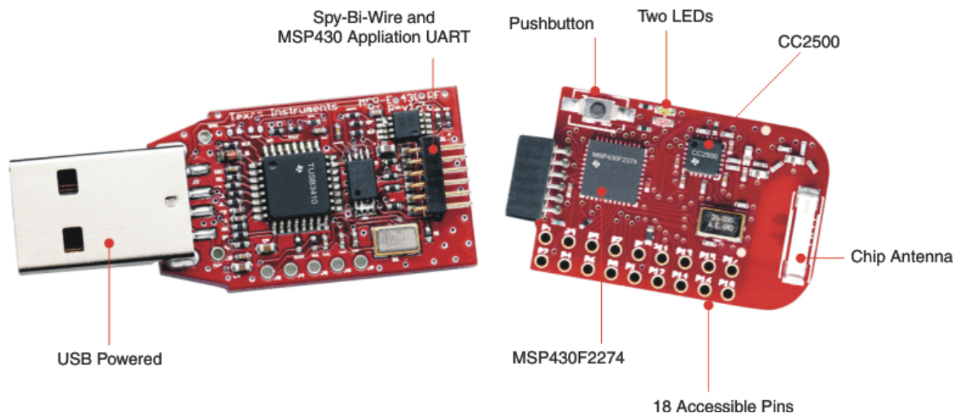
Figure 1. eZ430-RF2500
