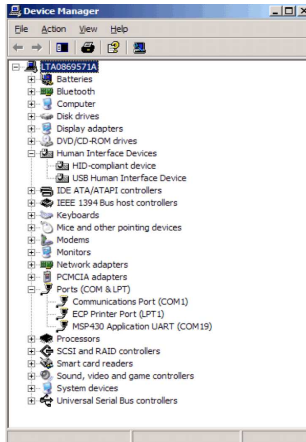
Figure 19. Device Manager
